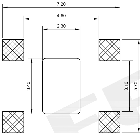
PCB LAYOUT
