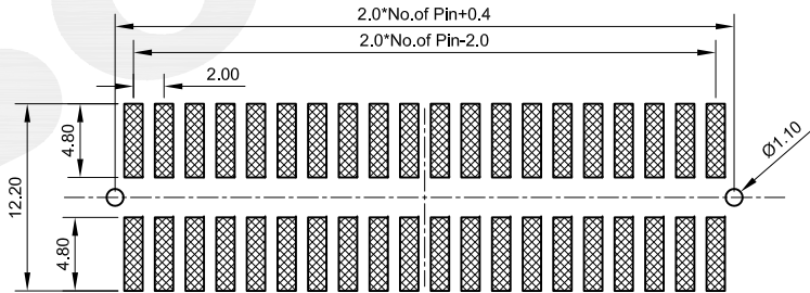
PCB LAYOUT
