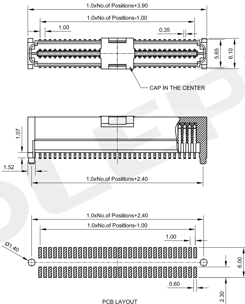
PCB LAYOUT
