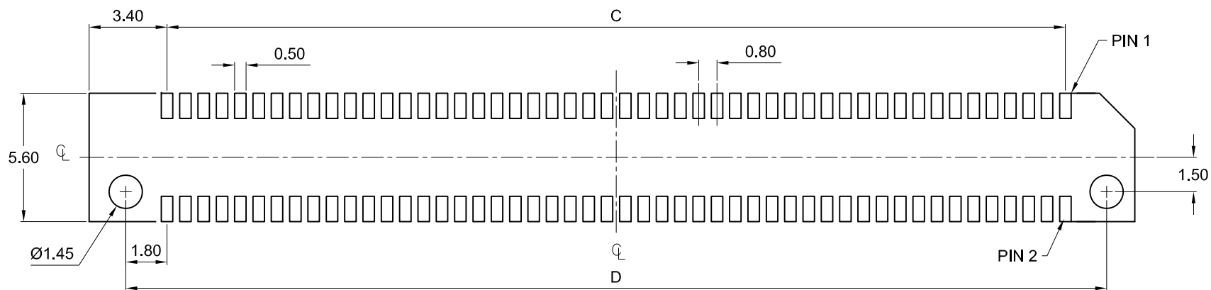
PCB LAYOUT
