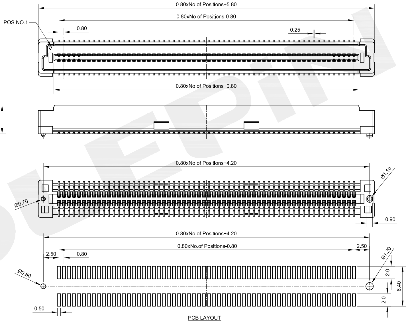
PCB LAYOUT
