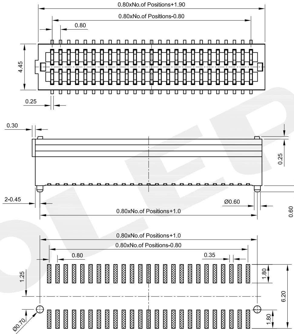
PCB LAYOUT
