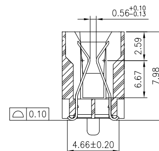
SECTION:A-A SCALE2:1
