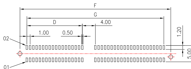
RECOMMENDED PCB LAYOUT(TOP SIDE) PCB BOARD TOLERANCE±0.05
