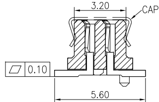
SECTION B-B W/T POST
