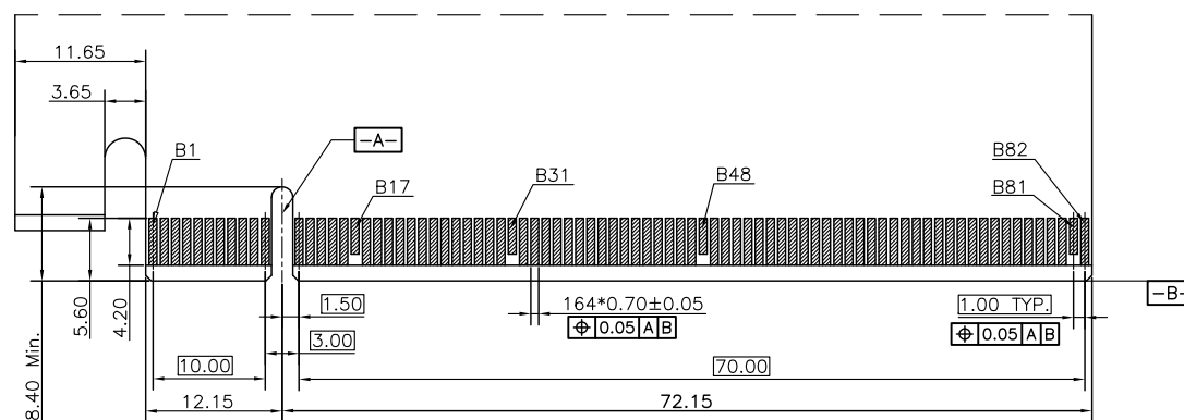
RECOMMENDED EDGE CARD PATTERN(PRIMARY SIDE)
