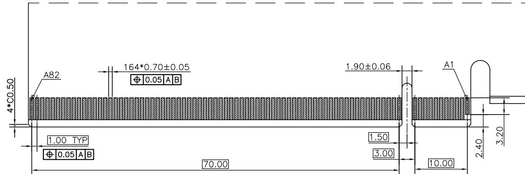
RECOMMENDED EDGE CARD PATTERN(SECONDARY SIDE)
