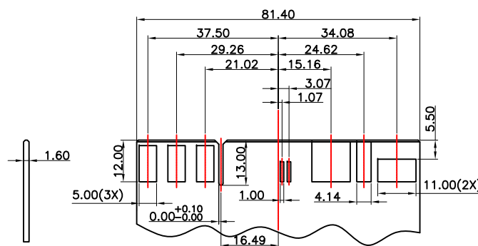
PCB RECOMMENDED HOLE SIZE DIAGRAM
