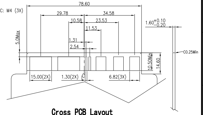
Cross PCB Layout
