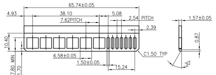
Recommended Edge Card Layout (Tolerance:±0.05)
